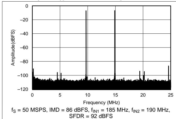
Figure 112. FFT for Two-Tone Input Signal (-7 dBFS at 185 MHz and 190 MHz)
