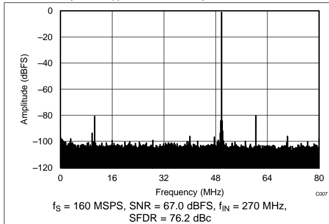
Figure 7. FFT for 270-MHz Input Signal (Dither On)
