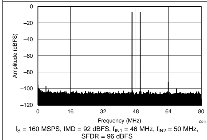
Figure 11. FFT for Two-Tone Input Signal ( -7\text{ dBFS} at 46 MHz and 50 MHz)
