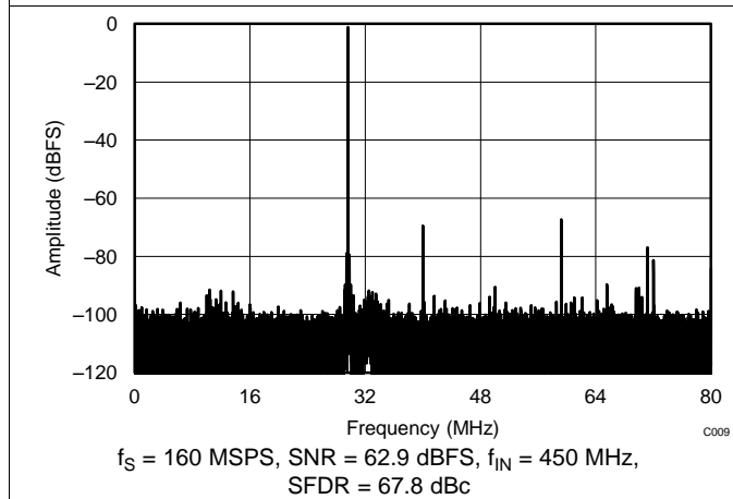
Figure 9. FFT for 450-MHz Input Signal (Dither On)
