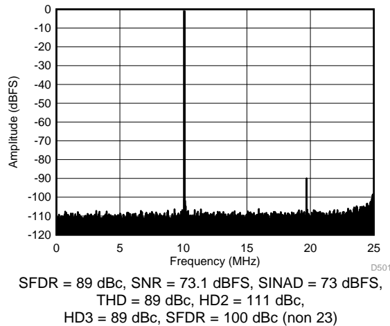
Figure 32. FFT for 10-MHz Input Signal (Dither On)
