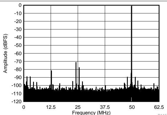
SFDR = 70 dBc, SNR = 68.9 dBFS, SINAD = 67.6 dBFS, THD = 73 dBc, HD2 = 77 dBc, HD3 = 70 dBc
