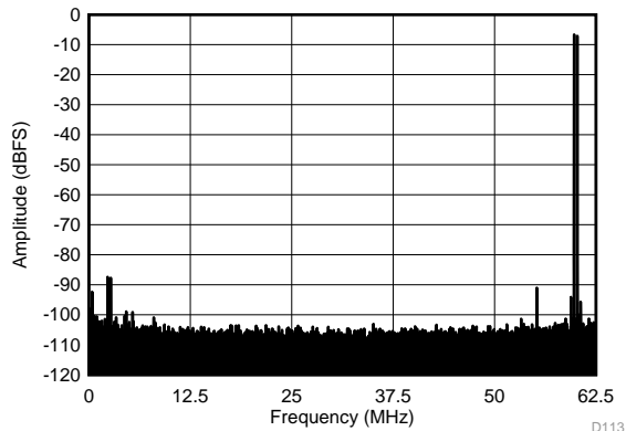
f_{IN1} = 185\text{ MHz} , f_{IN2} = 190\text{ MHz} , IMD3 = 88\text{ dBFS} , each tone at -7\text{ dBFS}
