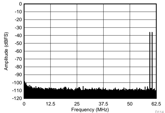
f_{IN1} = 185\text{ MHz} , f_{IN2} = 190\text{ MHz} , IMD3 = 104\text{ dBFS} , each tone at -36\text{ dBFS}
