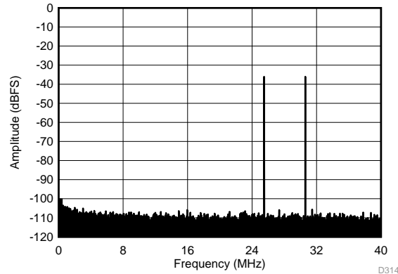
f_{IN1} = 185 \text{ MHz} , f_{IN2} = 190 \text{ MHz} , IMD3 = 106 dBFS, each tone at -36 dBFS
