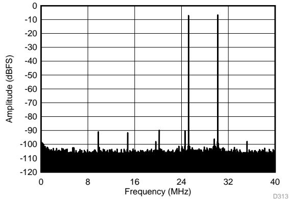
f_{IN1} = 185 \text{ MHz} , f_{IN2} = 190 \text{ MHz} , IMD3 = 90 dBFS, each tone at -7 dBFS
