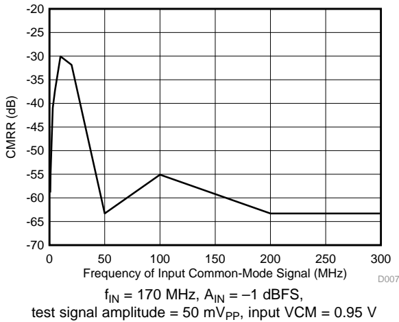
Figure 127. Common-Mode Rejection Ratio vs Test Signal Frequency
