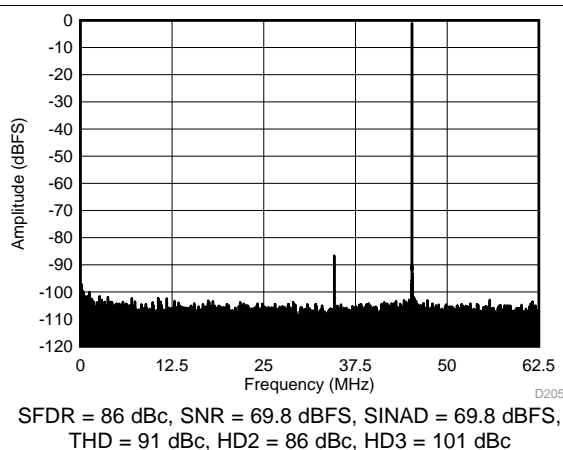
Figure 95. FFT for 170-MHz Input Signal (Dither On)
