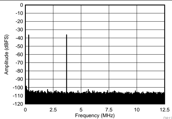
f_{IN1} = 46\text{ MHz} , f_{IN2} = 50\text{ MHz} , IMD3 = 105, each tone at = -36 dBFS
