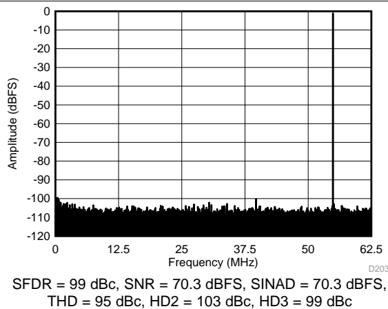
Figure 93. FFT for 70-MHz Input Signal (Dither On)
