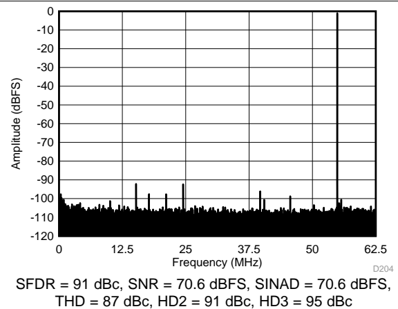
Figure 94. FFT for 70-MHz Input Signal (Dither Off)
