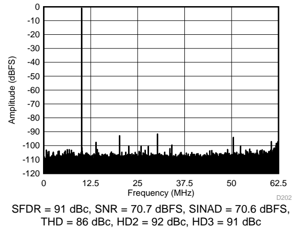
Figure 92. FFT for 10-MHz Input Signal (Chopper On, Dither Off)
