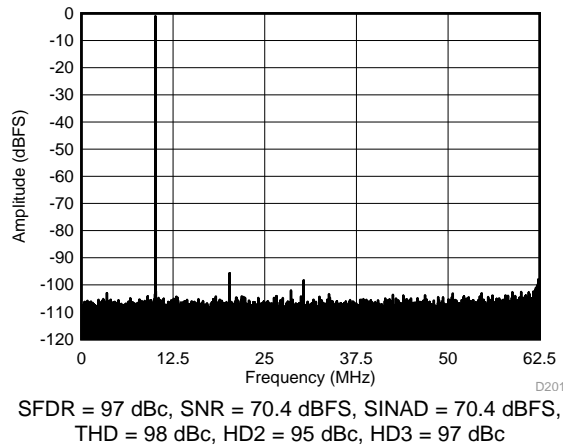
Figure 91. FFT for 10-MHz Input Signal (Chopper On, Dither On)
