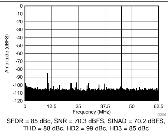
Figure 96. FFT for 170-MHz Input Signal (Dither Off)
