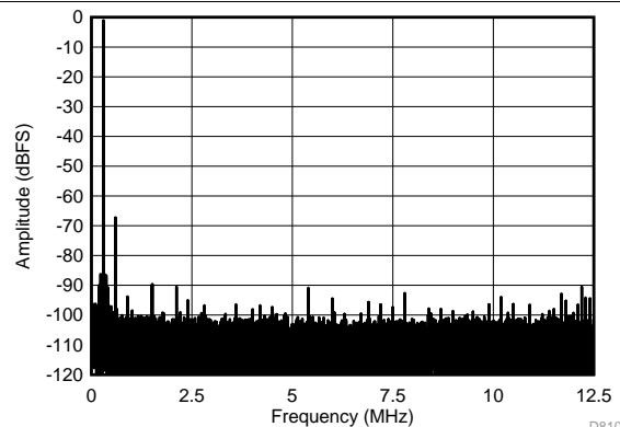
SFDR = 66 dBc, SNR = 66.5 dBFS, SINAD = 66.5 dBFS, THD = 87 dBc, HD2 = 66 dBc, HD3 = 93 dBc
