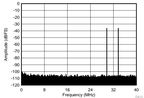
f_{IN1} = 46 \text{ MHz} , f_{IN2} = 50 \text{ MHz} , IMD3 = 105 dBFS, each tone at -36 dBFS
