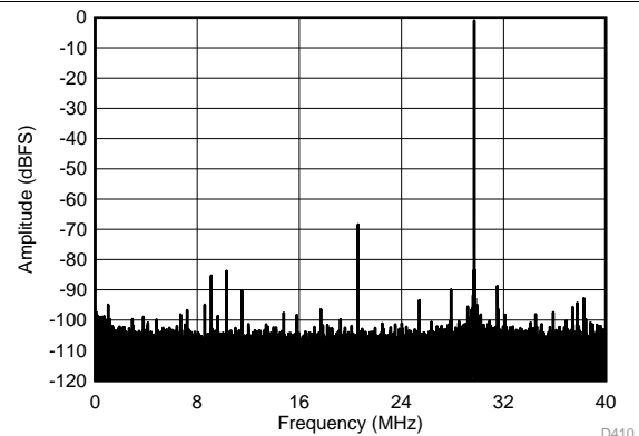
SFDR = 67 dBc, SNR = 67.7 dBFS, SINAD = 67.3 dBFS, THD = 77 dBc, HD2 = 67 dBc, HD3 = 84 dBc
