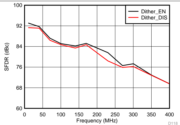
f_S = 160\text{ MSPS} , f_{IN} = 100\text{ MHz}
