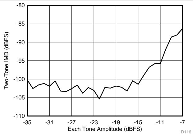
f_S = 160\text{ MSPS} , f_{IN1} = 185\text{ MHz} , f_{IN2} = 190\text{ MHz}
