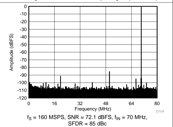
Figure 4. FFT for 70-MHz Input Signal (Dither Off)
