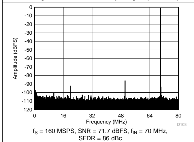
Figure 3. FFT for 70-MHz Input Signal (Dither On)
