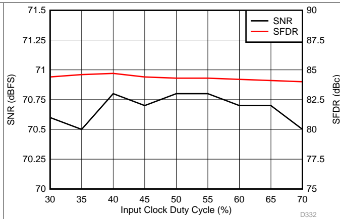
Figure 65. Performance vs Clock Duty Cycle (150 MHz)
