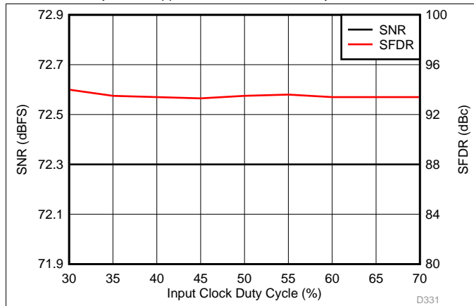
Figure 64. Performance vs Clock Duty Cycle (40 MHz)
