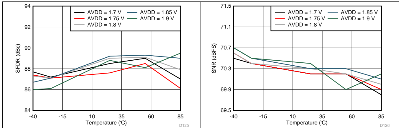
Figure 25. Spurious-Free Dynamic Range vs AVDD Supply and Temperature
