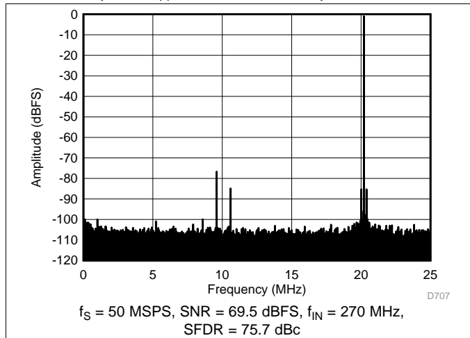
Figure 106. FFT for 270-MHz Input Signal (Dither On)
