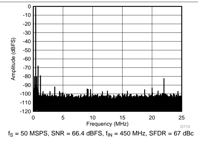
Figure 109. FFT for 450-MHz Input Signal (Dither Off)
