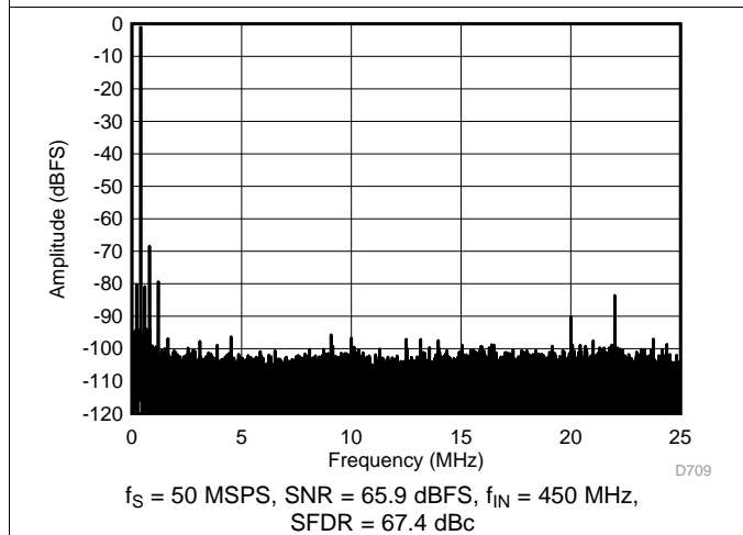
Figure 108. FFT for 450-MHz Input Signal (Dither On)
