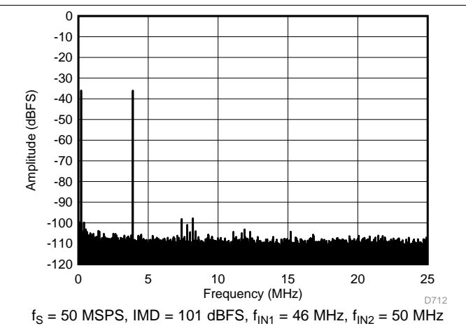
Figure 111. FFT for Two-Tone Input Signal (-36 dBFS at 46 MHz and 50 MHz)
