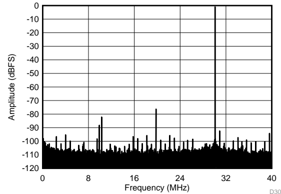
SFDR = 75.4 dBc, SNR = 71.2 dBFS, SINAD = 69.8 dBFS, THD = 74.2 dBc, HD2 = -75.4 dBc, HD3 = -81.2 dBc
