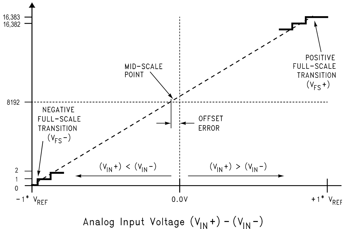
Figure 2. Transfer Characteristic
