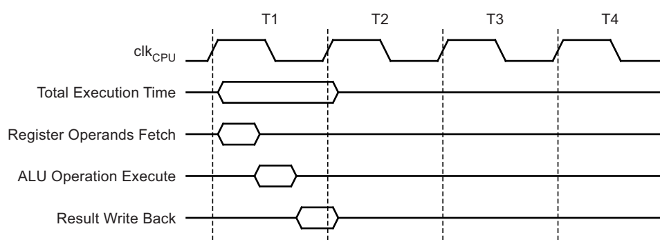
Figure 4-6. Single Cycle ALU Operation
