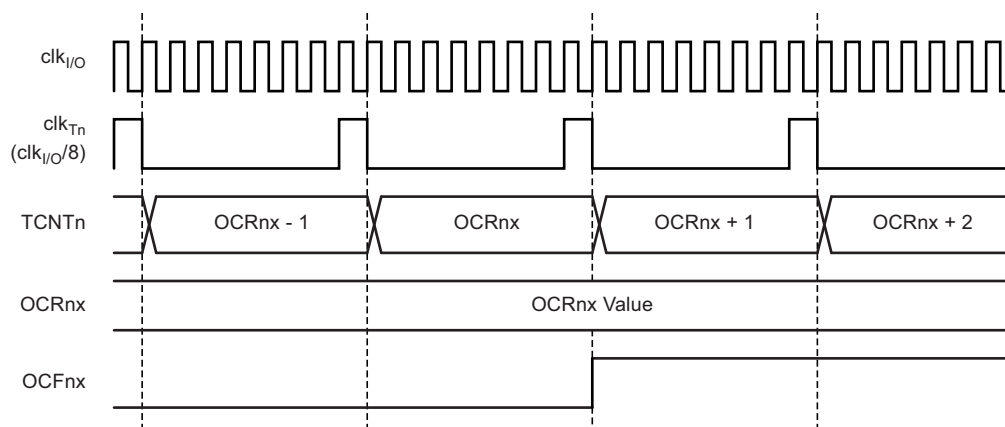
Figure 4-47. Timer/Counter Timing Diagram, Setting of OCF1x, with Prescaler ( f_{\text{clk\_I/O}}/8 )
