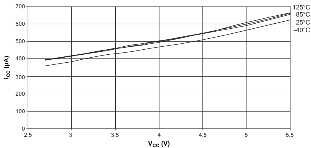
Figure 8-32. ADC Current versus V_{CC}
