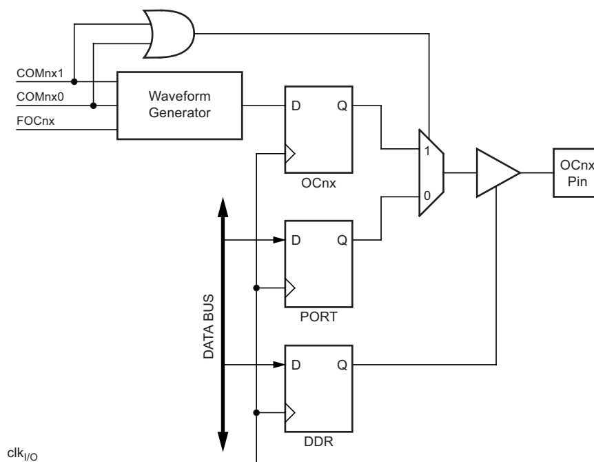
Figure 4-41. Compare Match Output Unit, Schematic
