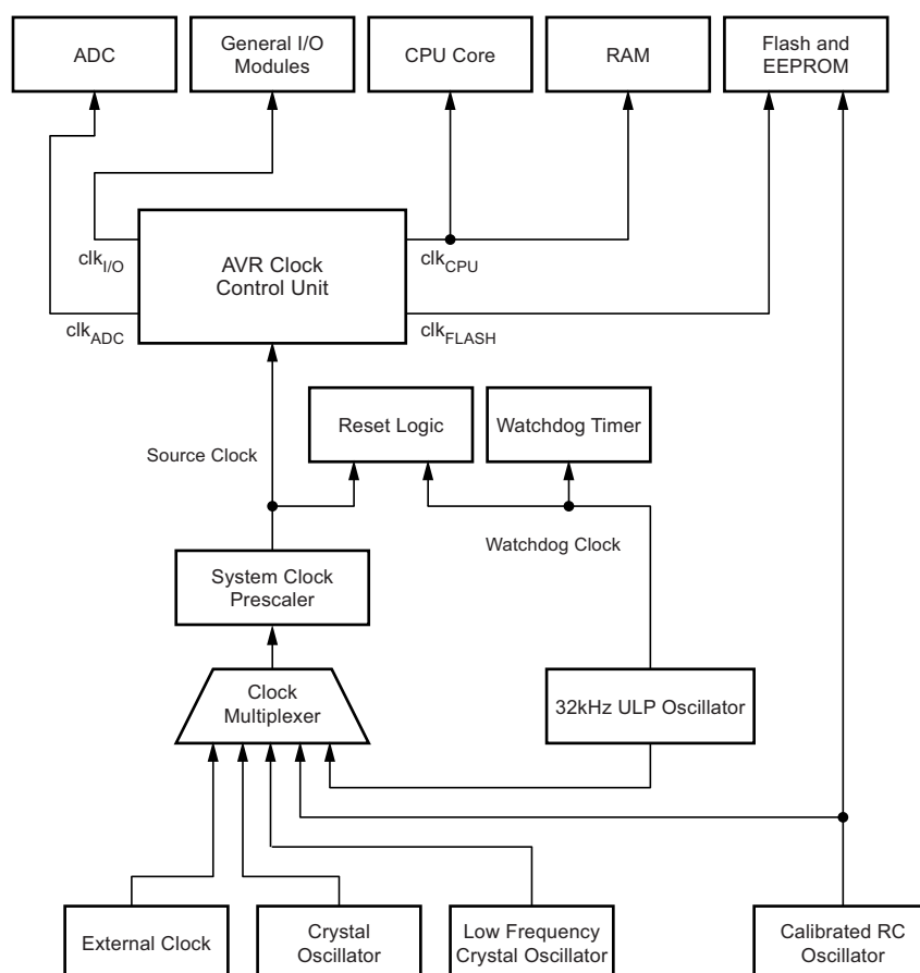
Figure 4-10. Clock Distribution
