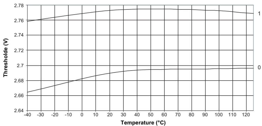
Figure 8-26. BOD Threshold versus Temperature (BODLEVEL is 2.7V)
