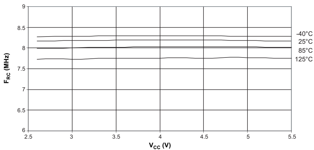
Figure 8-29. Calibrated 8MHz RC Oscillator Frequency versus V_{CC}
