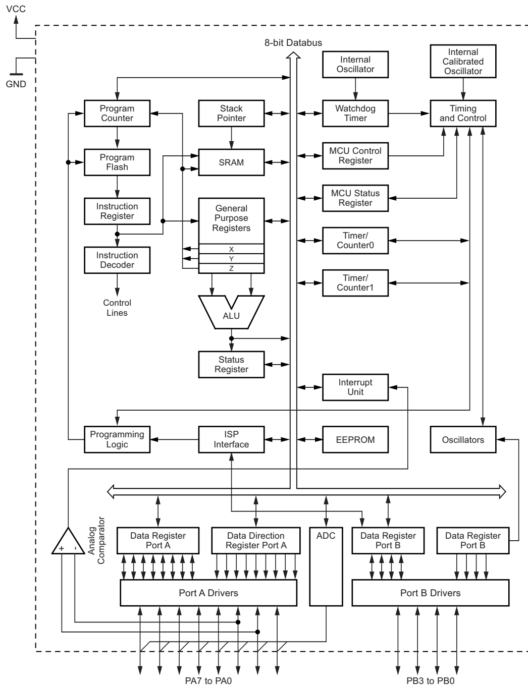
Figure 4-1. Block Diagram
