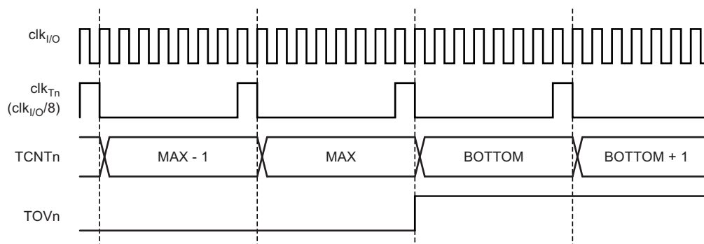
Figure 4-34. Timer/Counter Timing Diagram, with Prescaler ( f_{\text{clk\_I/O}}/8 )
