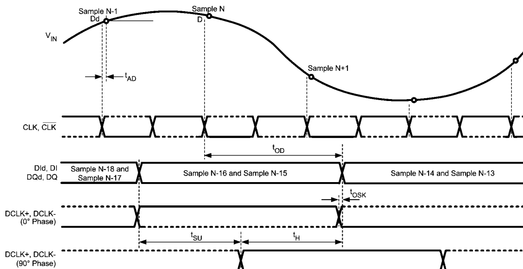
FIGURE 4. DDR Clcking in 1:2 Demultiplexed Non-DES Mode
