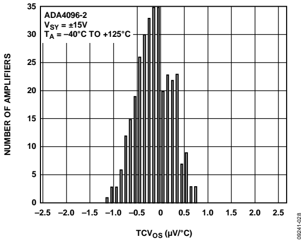
Figure 35. Offset Voltage Drift ( TCV_{OS} ) Distribution
