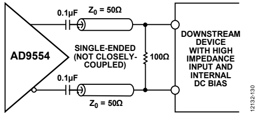
Figure 21. Destination Self-Biased Differential Receiver; Use 14 mA Mode for LVDS-Compatible Amplitude or 28 mA for LVPECL-Compatible Amplitudes (100 Ω resistor must be as close to the destination receiver as possible.)
