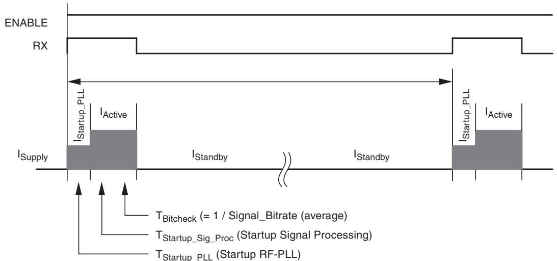
Figure 8-1. Polling Cycle
