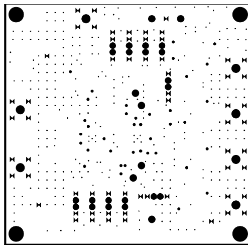
Figure 69. Ground Plane Copper
