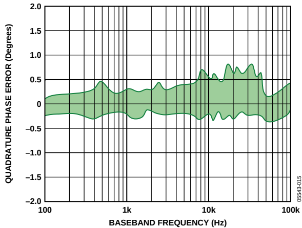
Figure 15. Representative Range of Quadrature Phase Error vs. Baseband Frequency, Channel 1 and Channel 2 (see Figure 43)
