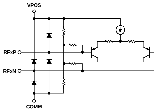
Figure 6. RF Inputs
