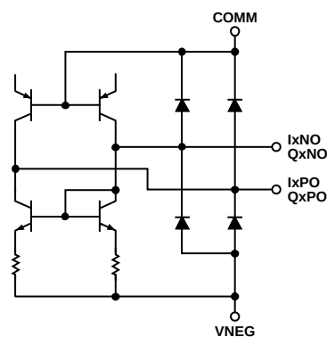
Figure 7. Output Drivers
