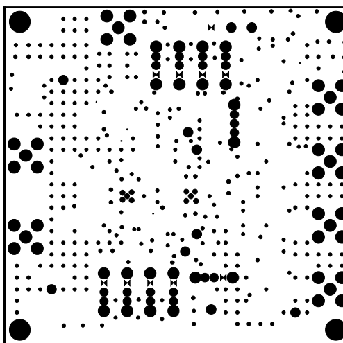
Figure 70. Power Plane Copper
