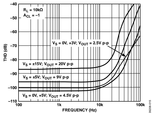
Figure 15. Total Harmonic Distortion (THD) vs. Frequency
