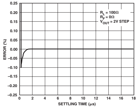
TPC 23. AD8047 Long-Term Settling Time, G = +1
