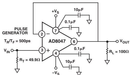
TPC 1. AD8047 Noninverting Configuration, G = +1
