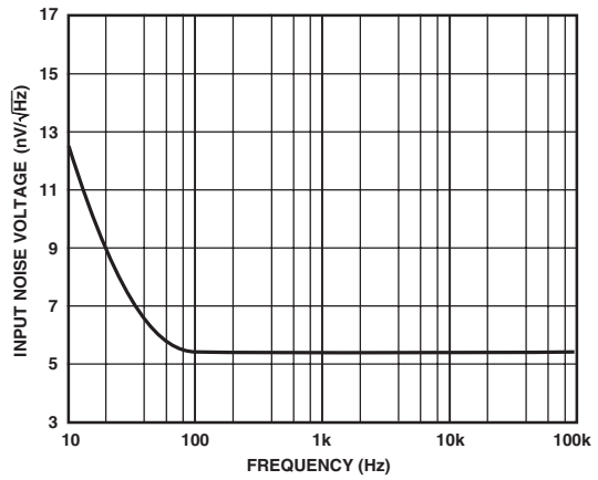
TPC 24. AD8047 Noise vs. Frequency
