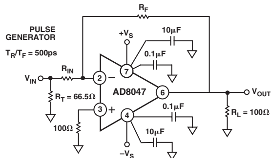
TPC 4. AD8047 Inverting Configuration, G = -1
