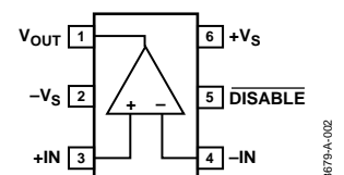
Figure 2. SC70-6 (KS)
