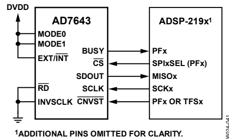
Figure 42. Interfacing the AD7643 to ADSP-219x
