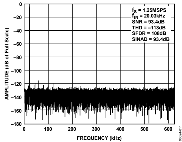
Figure 12. FFT 20 kHz
