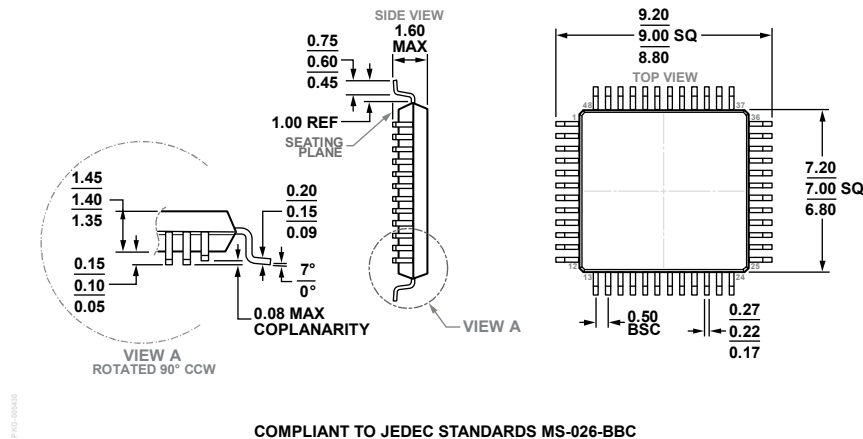
Figure 44. 48-Lead Low Profile Quad Flat Package [LQFP] (ST-48)
