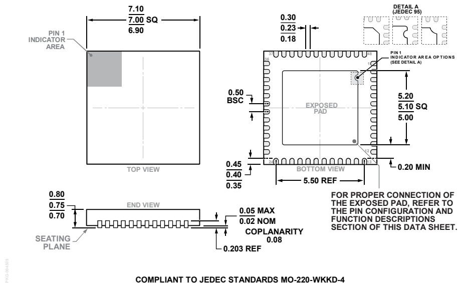
Figure 43. 48-Lead Lead Frame Chip Scale Package [LFCSP] 7 mm × 7 mm Body and 0.75 mm Package Height (CP-48-4)
