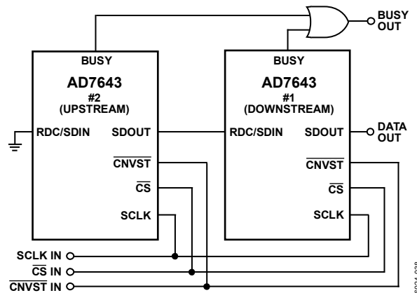
Figure 39. Two AD7643 Devices in a Daisy-Chain Configuration
