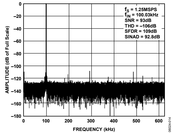
Figure 15. FFT 100 kHz
