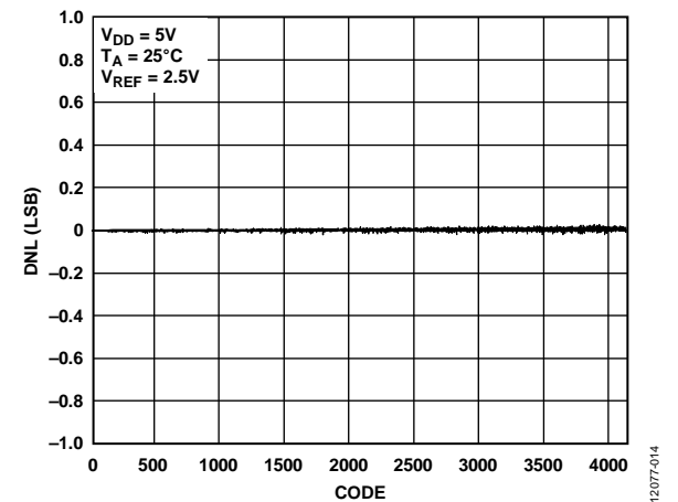
Figure 14. AD5691R DNL
