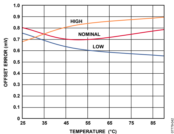
Figure 27. MV Offset Error vs. Temperature, MEASOUT Gain = 1
