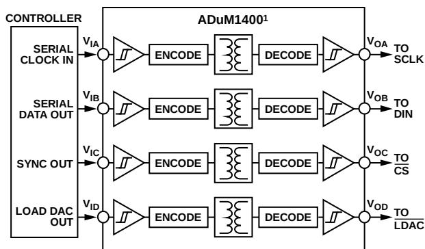
Figure 34. Isolated Interface
