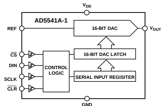
Figure 2. AD5541A-1
