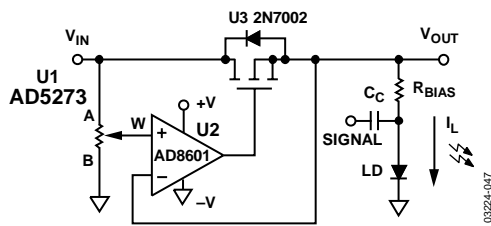
Figure 44. Programmable Booster Voltage Source
