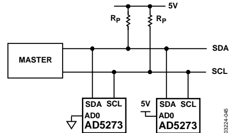
Figure 42. Two AD5273 Devices on One Bus
