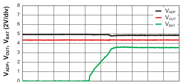
Time (200μs/div)
