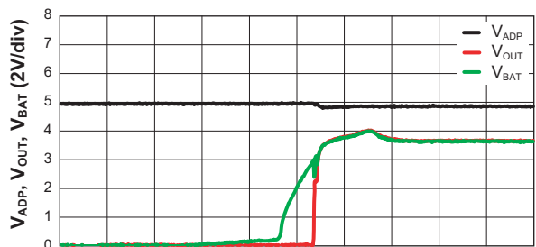
Time (200μs/div)
