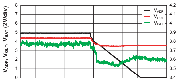
Time (200µs/div)
