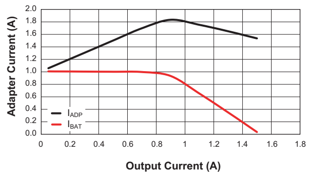
Adapter Charging Current vs. Output Current
