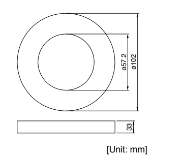
Fig.3: T400-61D (Recommended components)
