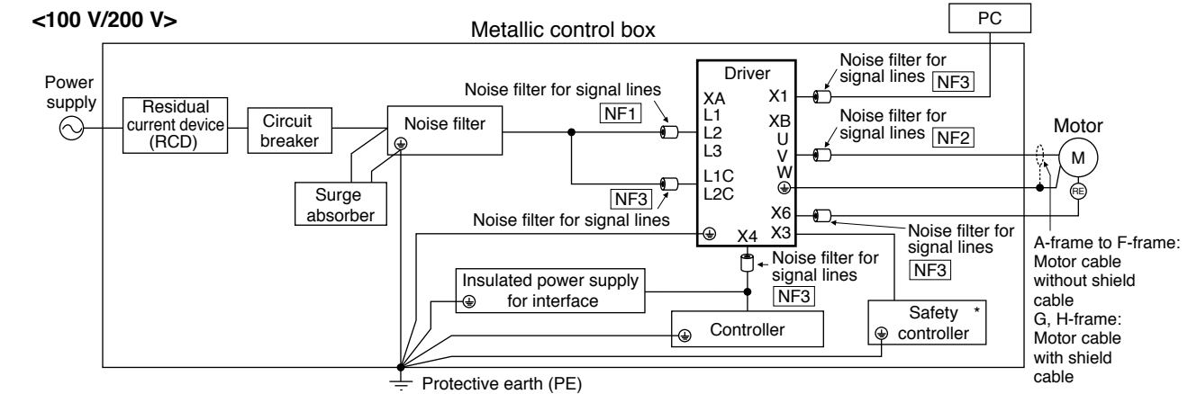
For [NF1] to [NF3], refer to the Table “Noise Filter for Signal Line” (P.254). * A5IE, A5E is not provided with X3 terminal.
