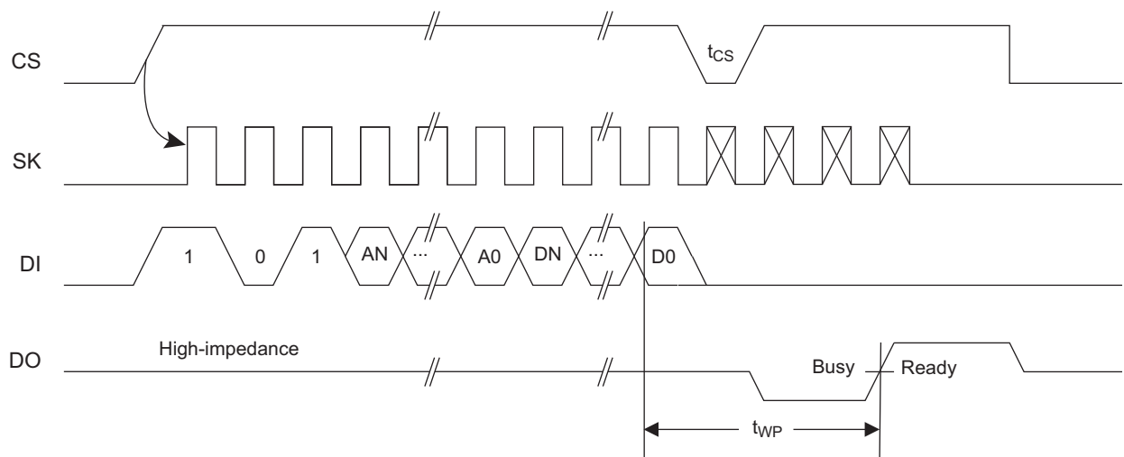
Figure 6-5. WRITE Timing
