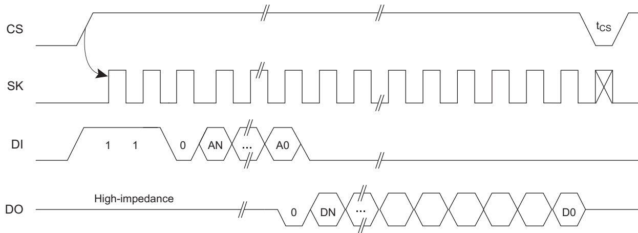
Figure 6-3. READ Timing
