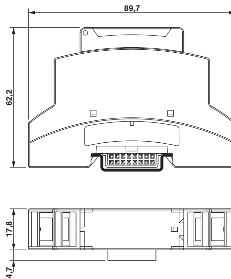
Dimensioned drawing
