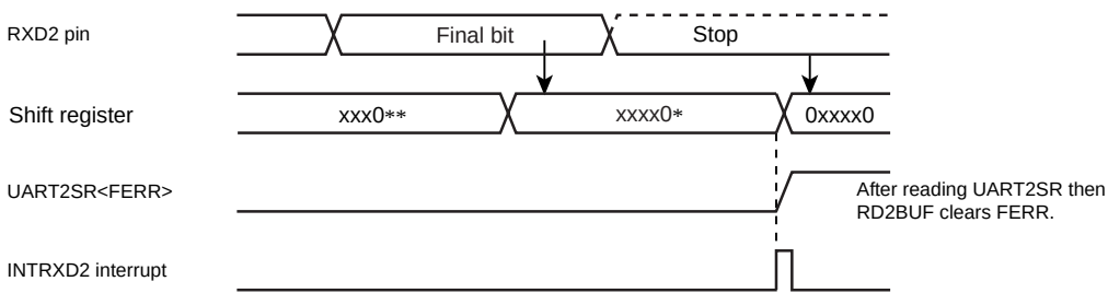
Figure 13-6 Generation of Framing Error
