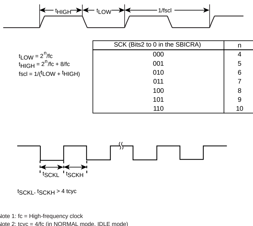
Figure 15-3 Clock Source
