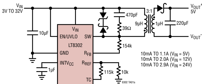
3V to 32V IN /5V OUT Isolated Flyback Converter
