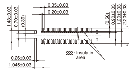
Recommended metal mask pattern Metal mask thickness: When 100 \mu m (Signal terminal opening ratio: 70%) (Power terminal opening ratio: 77%)
