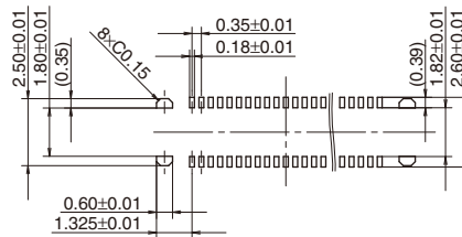
Recommended metal mask pattern Metal mask thickness: When 100 \mu m (Terminal opening ratio: 70%) (Metal-part opening ratio: 46%)
