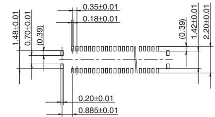
Recommended metal mask pattern Metal mask thickness: When 100 \mu m (Signal terminal opening ratio: 70%) (Power terminal opening ratio: 77%)
