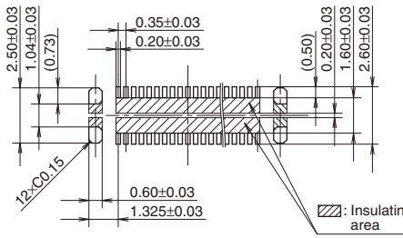
Recommended metal mask pattern Metal mask thickness: When 100 \mu m (Terminal opening ratio: 70%) (Metal-part opening ratio: 46%)
