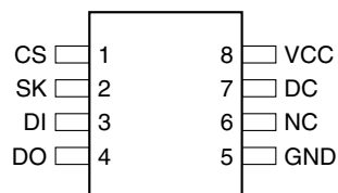
8-lead SOIC
