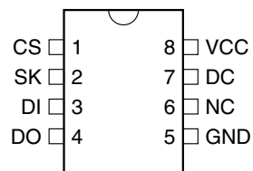
8-lead PDIP
