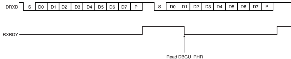
Figure 28-6. Receiver Ready
