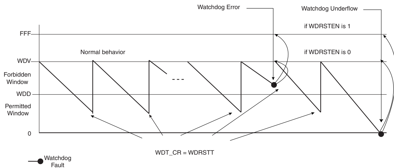
Figure 16-2. Watchdog Behavior
