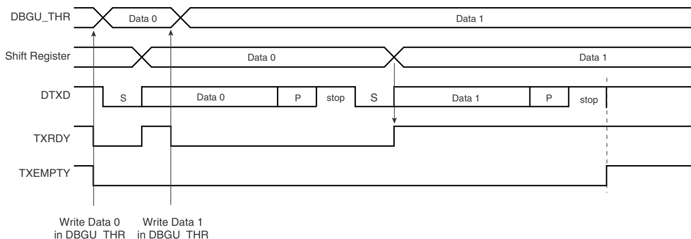
Figure 28-11. Transmitter Control
