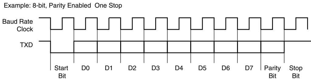
Figure 32-6. Character Transmit
