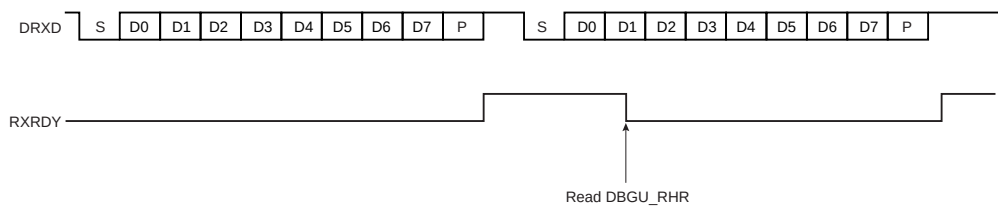
Figure 23-6. Receiver Ready
