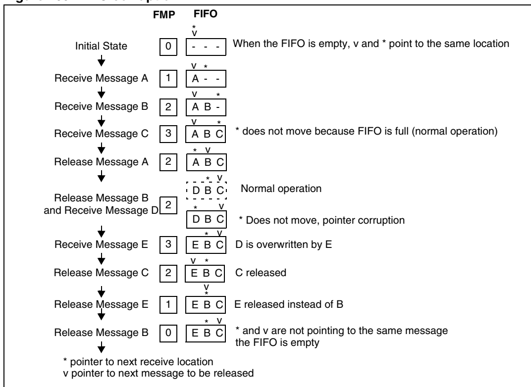
Figure 109. FIFO corruption
