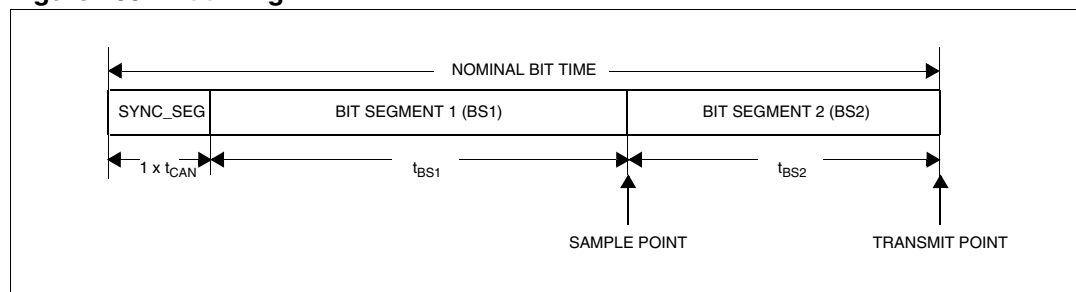
Figure 105. Bit timing
