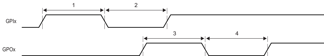
Figure 11-52. GPIO Timing
