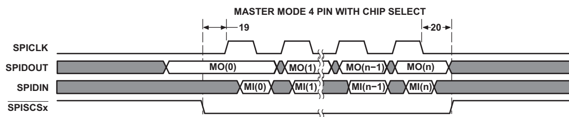
Figure 5-12. SPI Additional Timings for 4-Pin Master Mode With Chip Select Option
