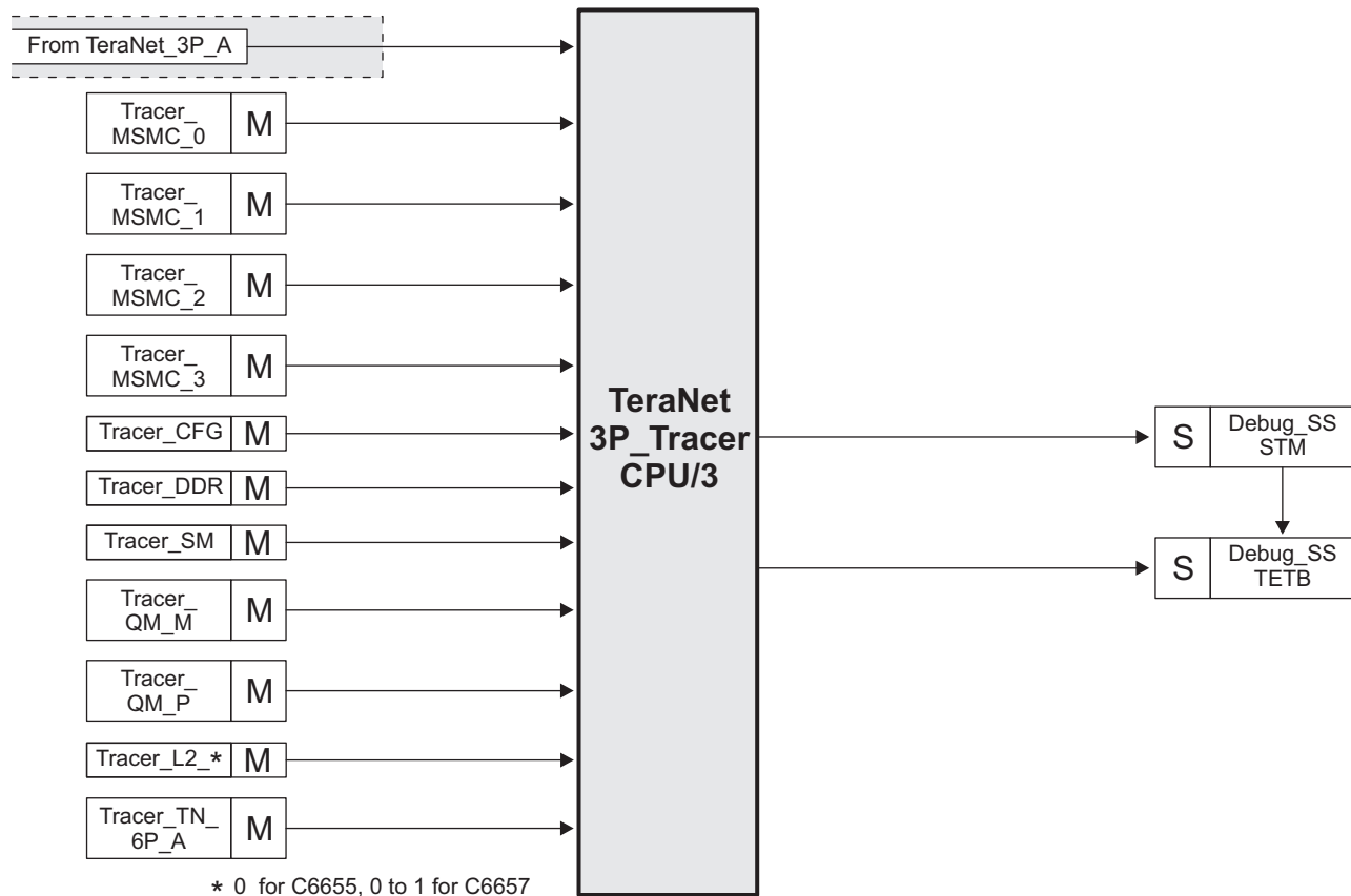
Figure 9-4. TeraNet 3P_Tracer
