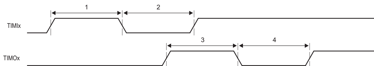
Figure 5-26. Timer Timing
