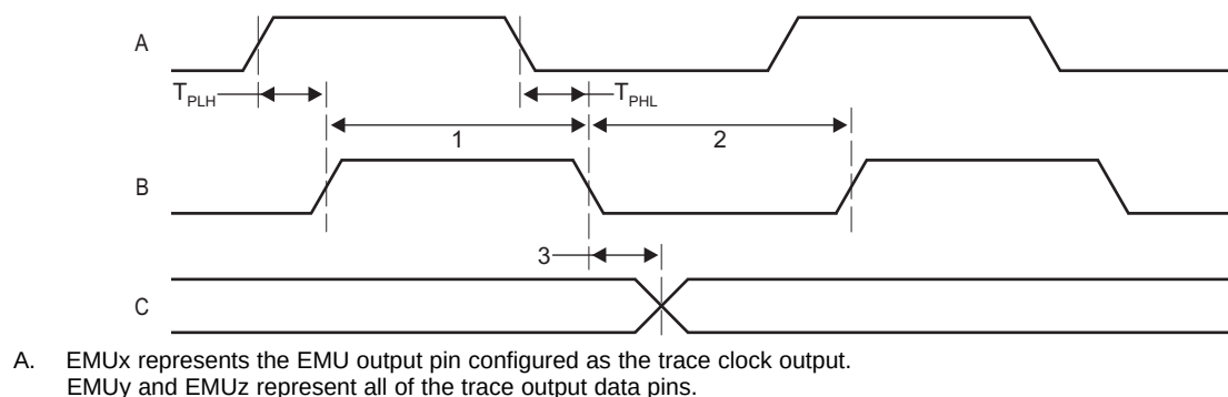
Figure 5-34. Trace Timing
