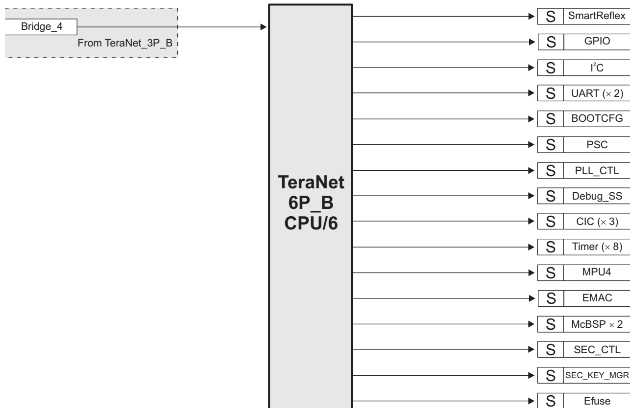
Figure 9-5. TeraNet 6P_B
