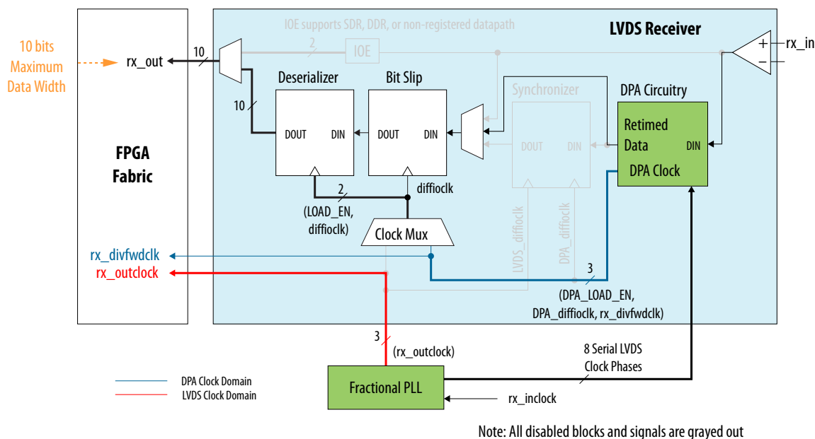
Figure 6-26: Receiver Datapath in Soft-CDR Mode
