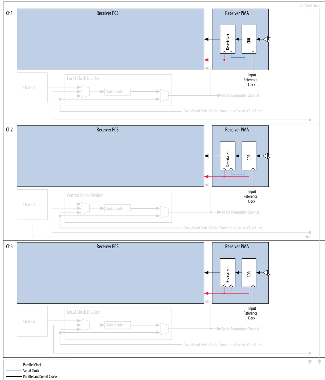
The figure shows three channels configured in non-bonded configuration. They use the receiver standard PCS that does not use a rate match FIFO. The CDR of each channel recovers the serial clock (recovered) from the incoming data and generates the parallel clock (recovered) by dividing the serial clock (recovered). Depending on the configuration, the receiver PCS may also use the parallel clock from the clock divider that is generated by the local clock divider for the transmitter.
