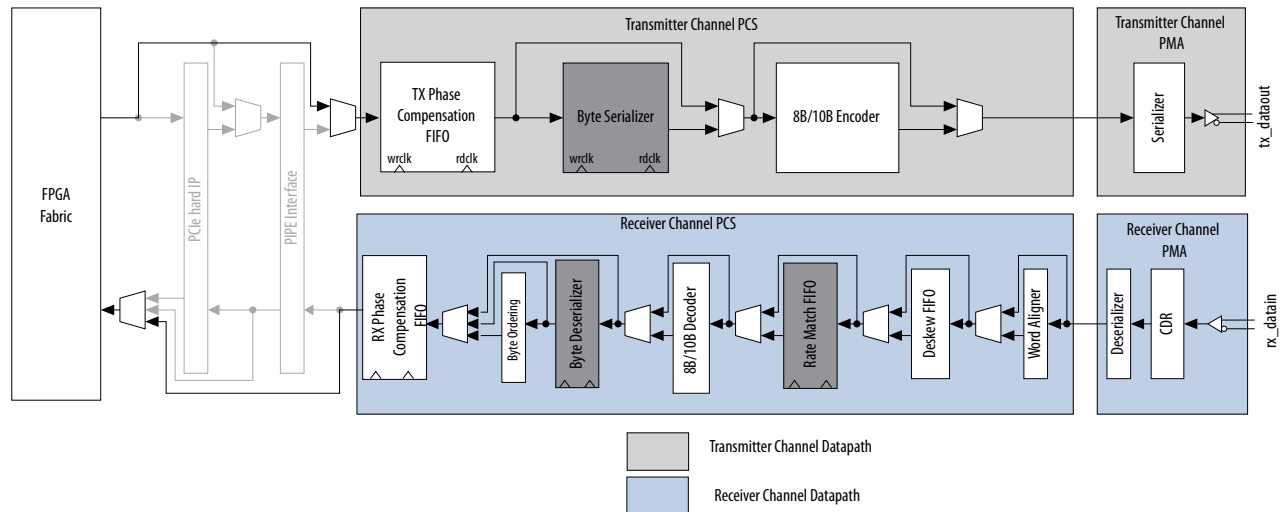
Figure 4-49: Transceiver Datapath in Deterministic Latency Mode
