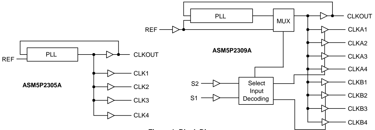
Figure 1. Block Diagram
