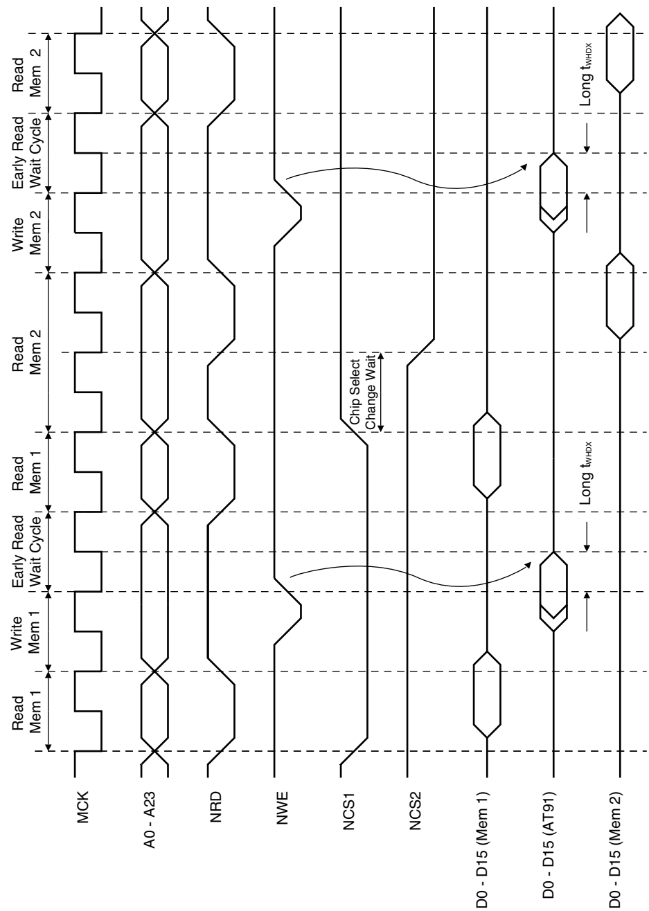
Figure 11-16. Early Read Protocol with no t_{DF}
