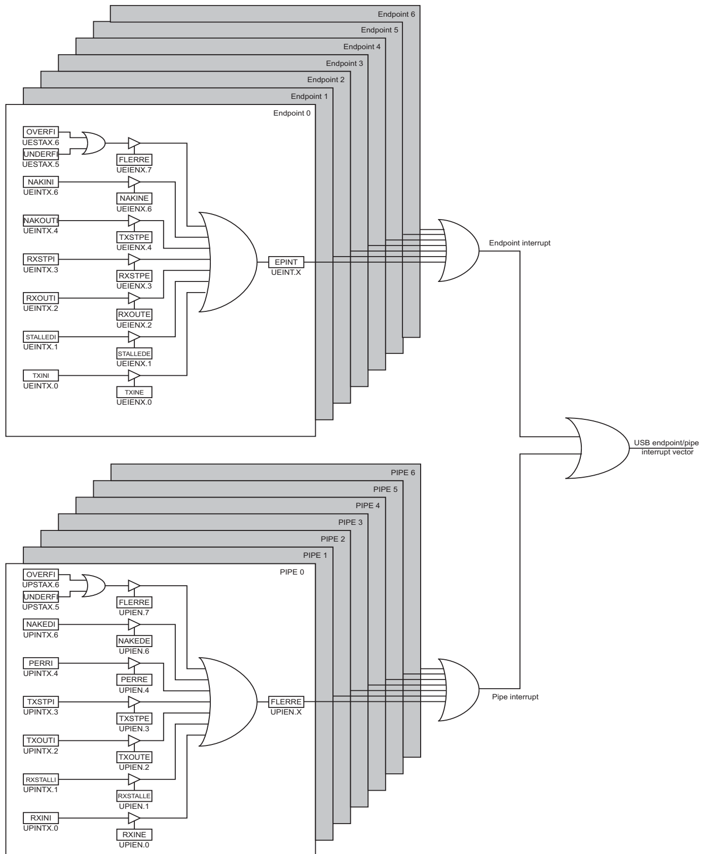
Figure 22-12. USB endpoint/pipe Interrupt vector sources.
