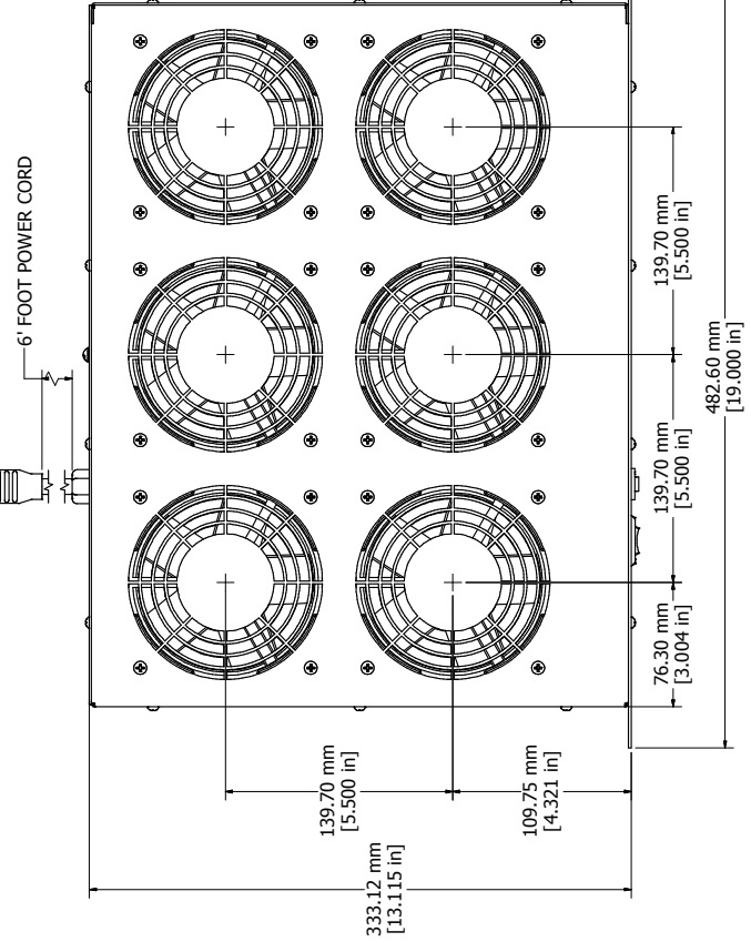
ASSEMBLY - VIEW FROM TOP
