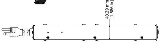
ASSEMBLY - VIEW FROM SIDE
