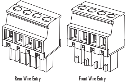
Rear Wire Entry
