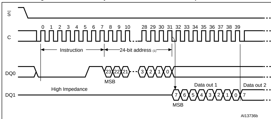
Figure 11. Read Data Bytes instruction and data-out sequence
