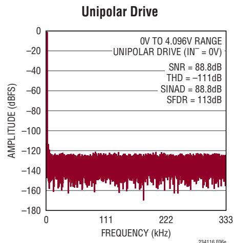
Figure 6e. IN^+ = -1\text{dBFS} 2kHz Unipolar Sine, IN^- = 0\text{V} , 32k Point FFT, f_{\text{SAMPL}} = 666\text{ksps} . Circuit Shown in Figure 6a with LT6237 Amplifiers, R_{\text{FILT}} = 24.9\Omega , C_{\text{FILT}} = 1\text{nF}
