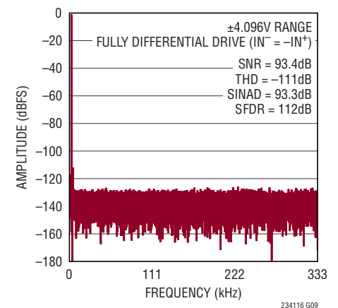
32k Point FFT f_{SAMPL} = 666\text{kHz} , f_{IN} = 2\text{kHz}
