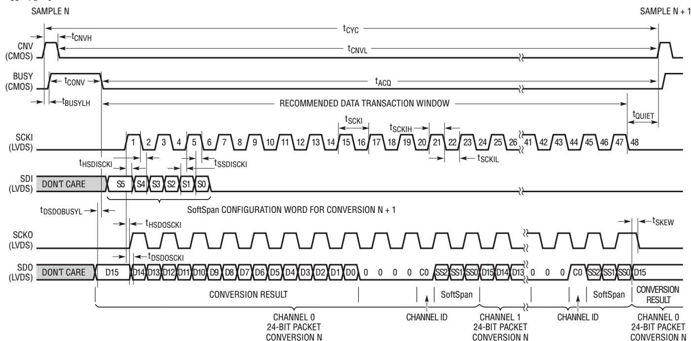
Figure 20. Serial LVDS I/O Mode
