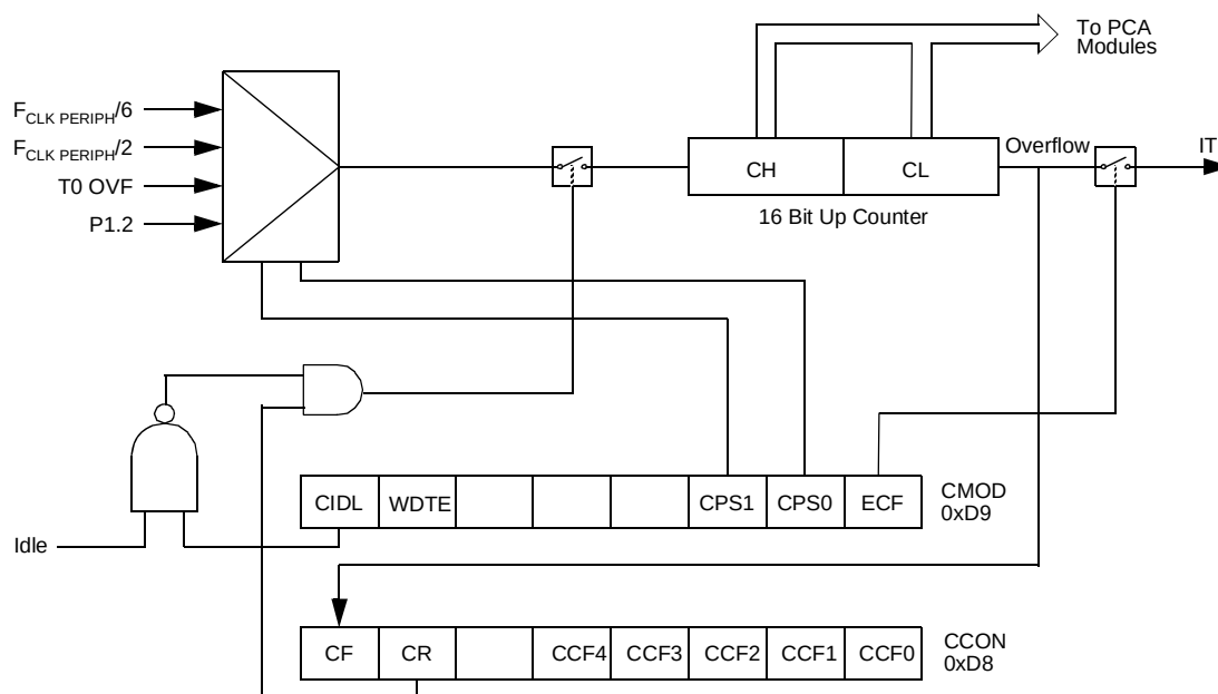
Figure 16. PCA Timer/Counter
