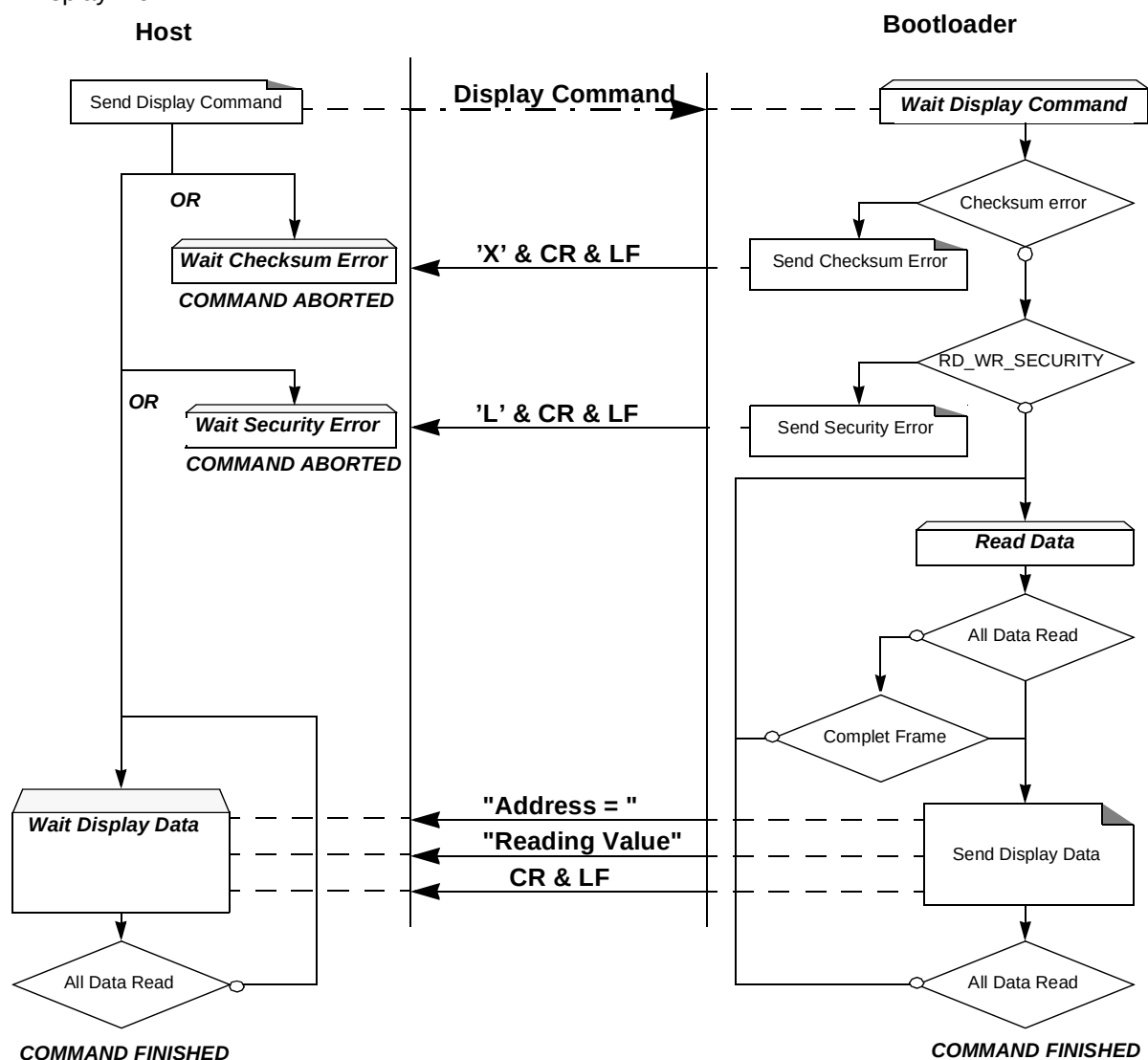
Figure 50. Display Flow
